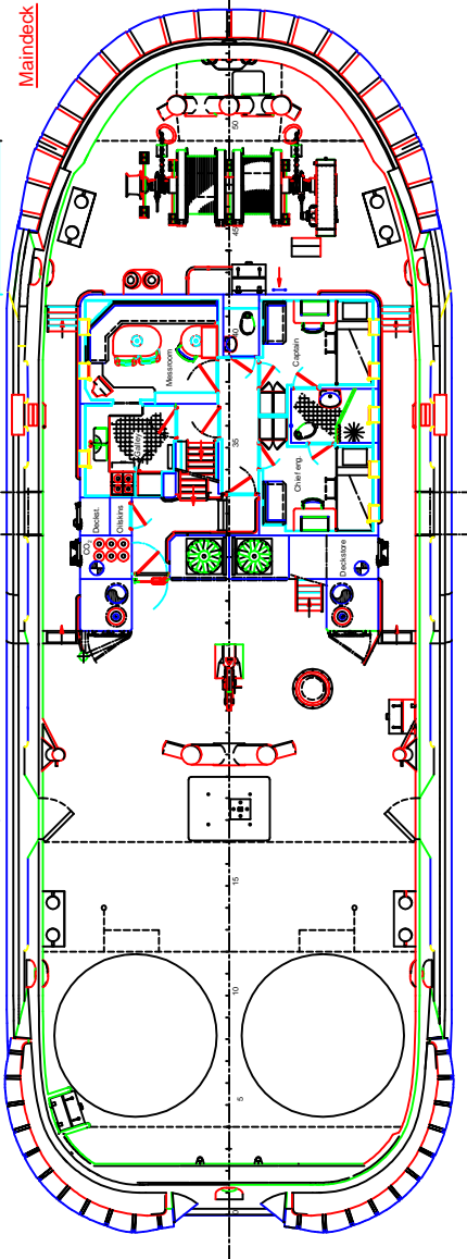
Below Maindeck
