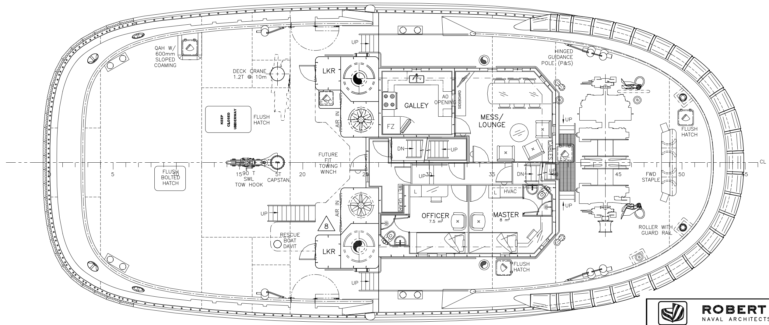
MAIN DECK
